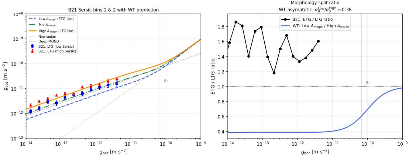
FIG. 8. Left: B21 Sérsic bins 1 (blue squares, LTG) and 2 (red triangles, ETG) with WT morphology curves. Right: observed ETG/LTG ratio from B21 (black circles) versus WT predicted g_{\text{obs}}^{\text{Low } A_{\text{morph}}} / g_{\text{obs}}^{\text{High } A_{\text{morph}}} ratio (blue curve). The WT prediction is < 1 throughout (LTG exceeds ETG), whereas the observed B21 ratio is > 1 . B21 attribute this inversion to hot circumgalactic gas in ETGs that inflates their apparent g_{\text{obs}} relative to their stellar-mass-based g_{\text{bar}} . Correcting ETG g_{\text{bar}} for hot gas is predicted to collapse the ratio toward the WT-ordered curve.
