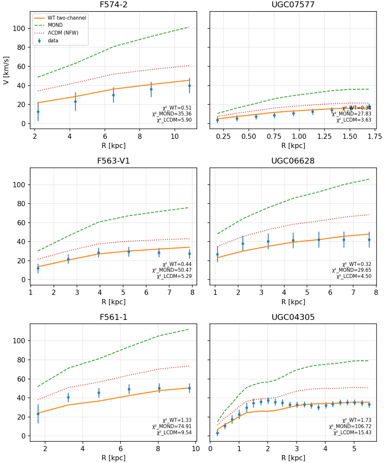
FIG. 4. G1 dwarfs at fixed \alpha_0 = 0.3 . F574-2, UGC07577, F563-V1, UGC06628, F561-1, and UGC04305 represent the most extended, lowest surface-brightness systems in the sample. All six panels use the same \alpha_0 = 0.3 ; annotated \chi^2 values for WT, MOND and \Lambda CDM are shown in each panel. The suppressed coupling is physically interpretable: where orbital phase mixing is least complete, the shell projection efficiency is accordingly reduced below the ideal disc baseline.
