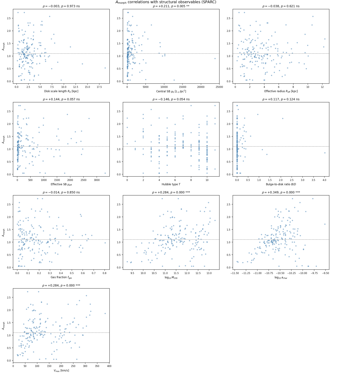
FIG. 9. Spearman scatter plots of A_{\text{morph}} against ten structural and dynamical observables for all 175 SPARC galaxies. Each panel annotates the Spearman \rho and p -value. Significant correlations ( p < 0.05 ): central disk surface brightness \mu_0 ( \rho = +0.21 , p = 0.005 ), \log_{10} M_{200} ( \rho = +0.28 , p < 0.001 ), \log_{10} a_{\text{char}} ( \rho = +0.35 , p < 0.001 ), and V_{\text{max}} ( \rho = +0.28 , p < 0.001 ). Non-significant ( p > 0.05 ): disk scale length R_d , effective radius R_{\text{eff}} , effective surface brightness, bulge-to-disk ratio B/D , Hubble type T , and gas fraction f_{\text{gas}} . The dashed line marks the universal \kappa prediction. The pattern confirms that A_{\text{morph}} tracks the central baryonic concentration rather than the total extent, morphological class, or gas content of the galaxy.
