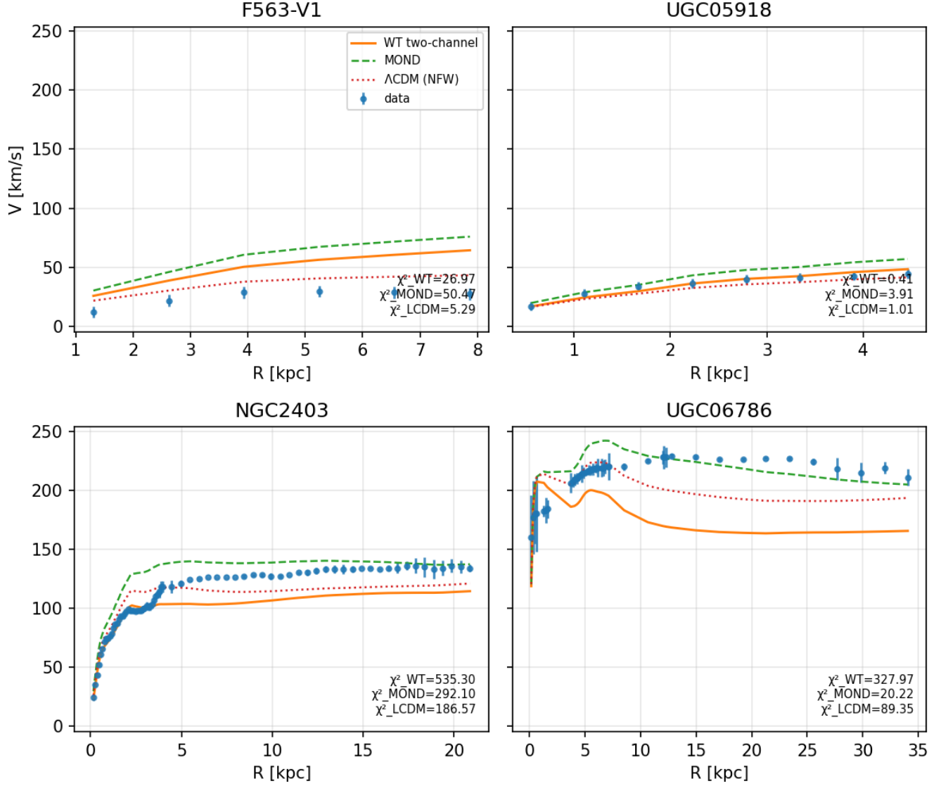
FIG. 5. One representative per calibration bin, all plotted at universal \kappa (zero free parameters). From left to right: F563-V1 (G1, A_{\text{morph}} = 0.23 ), UGC05918 (G2, 0.97), NGC2403 (G3, 1.55), UGC06786 (G4, 2.23). The A_{\text{morph}} values identify the bin of each representative (Table III); all curves use \alpha_0 = \kappa with no per-galaxy tuning. Each panel shows WT (solid), MOND (dashed), and \Lambda CDM NFW (dotted). The progressively later shell-coupling onset with increasing compactness is visible in the curvature of the rising inner section. Per-galaxy optimal fits are shown in Figures 3 and 4.
