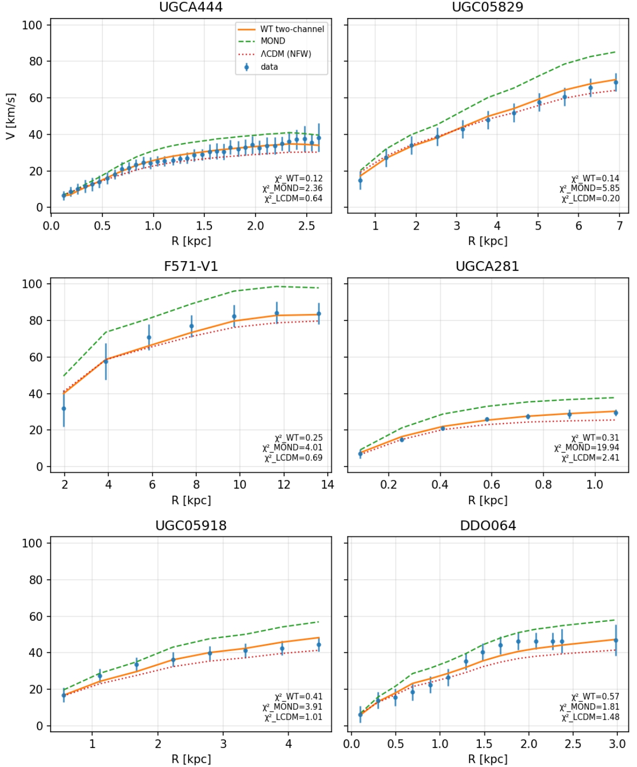
FIG. 2. Six best fits at universal \kappa = 1 + 1/\pi^2 . Galaxies UGCA444, UGC05829, F571-V1, UGCA281, UGC05918, and DDO064 achieve \chi^2_{WT} < 0.6 at the zero-parameter setting. All span the dwarf-to-intermediate mass range ( V_{\max} = 30\text{--}73\text{ km s}^{-1} , A_{\text{morph}} \approx 0.93\text{--}1.12 ), confirming that the formula is accurate throughout the low-acceleration regime where the shell channel dominates. The WT curves track the data through the rising inner region and into the flat outer tail without requiring any parameter adjustment.
