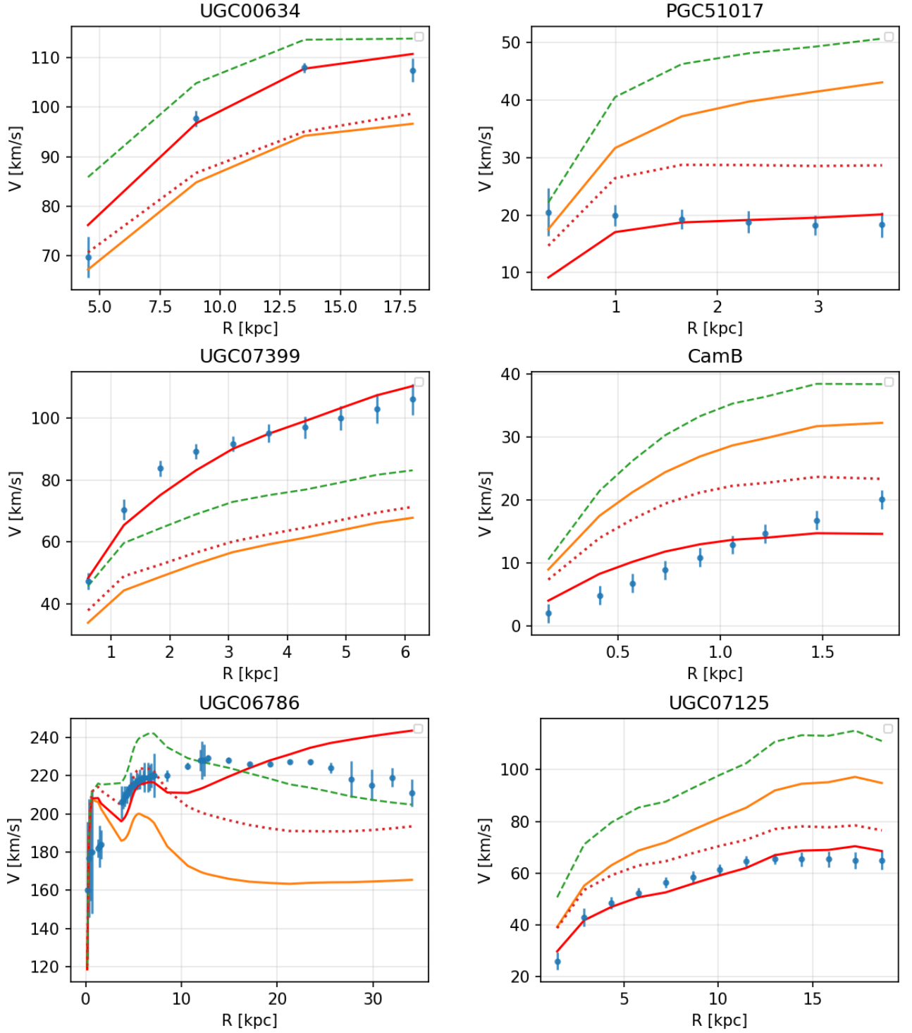
FIG. 3. Six galaxies spanning the full A_{\text{morph}} range (Table IV), from suppressed (PGC51017, CamB; A_{\text{morph}} = 0.19\text{--}0.21 ) through enhanced (UGC00634; 1.32) to high-coupling (UGC07399, UGC06786; 2.23–2.72). Orange: universal \kappa ( \chi^2 > 70 ); red: fitted \alpha_0 ( \chi^2 < 10 ). The gap between them quantifies the morphology correction; the formula shape is correct in all six cases.
