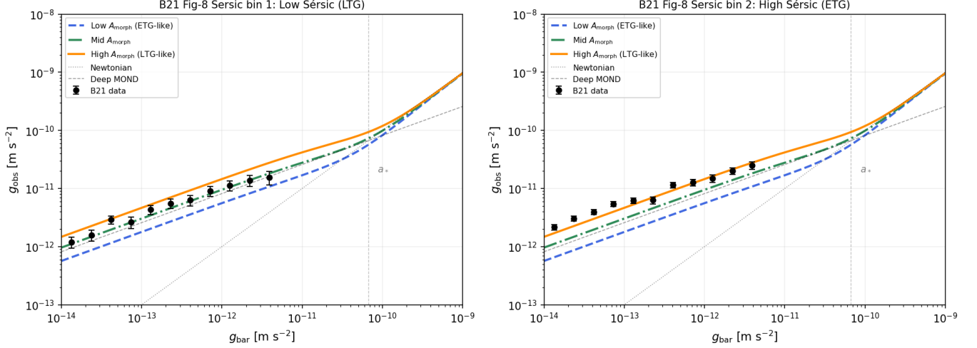
WT morphology prediction vs Brouwer+2021 (KiDS-1000) Sérsic split Low A_{\text{morph}} \rightarrow \text{ETG} ; High A_{\text{morph}} \rightarrow \text{LTG} | Predicted ratio: \alpha_0^{\text{High}}/\alpha_0^{\text{Low}} = 2.60
